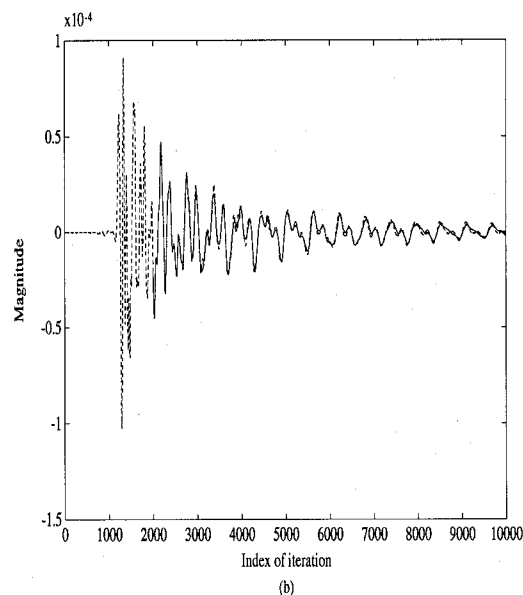
Figure 2: AR curve fitting and extrapolation compared with FD-TD method. — FD-TD + AR method - - FD-TD records
