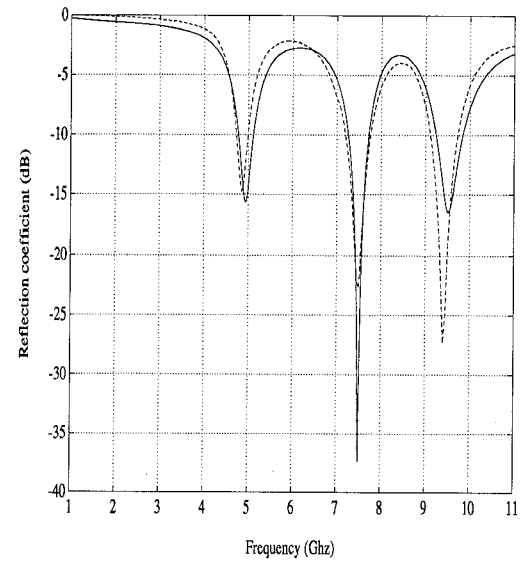
Figure 5: Reflection coefficient of the coaxial-fed patch antenna. — 1-2500 FD-TD records plus AR method. - - measurement result.
